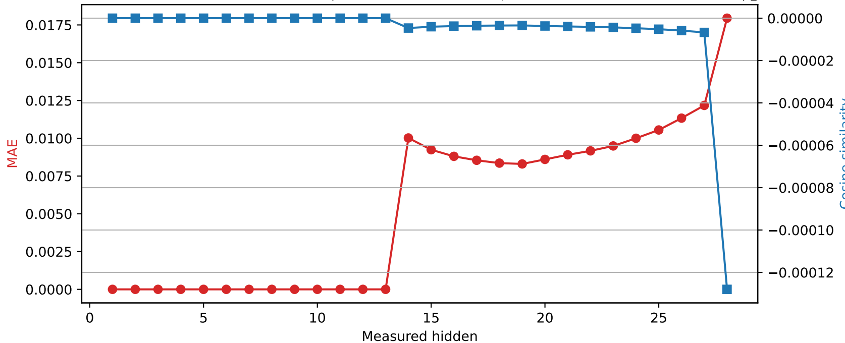
Llama-3.2-3B | Quantized layer 13 | float16 → int8
