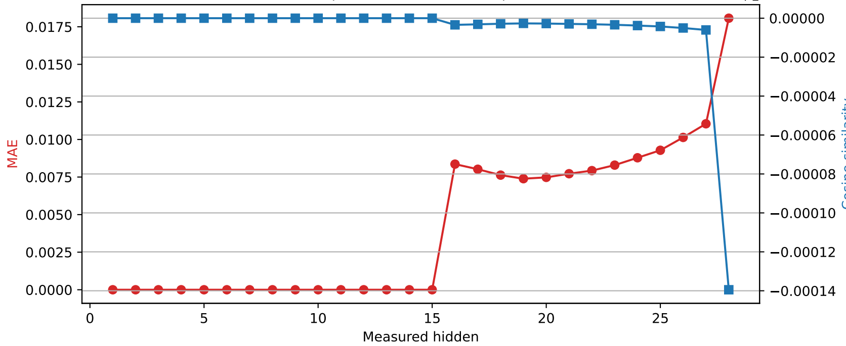
Llama-3.2-3B | Quantized layer 15 | float16 → int8
