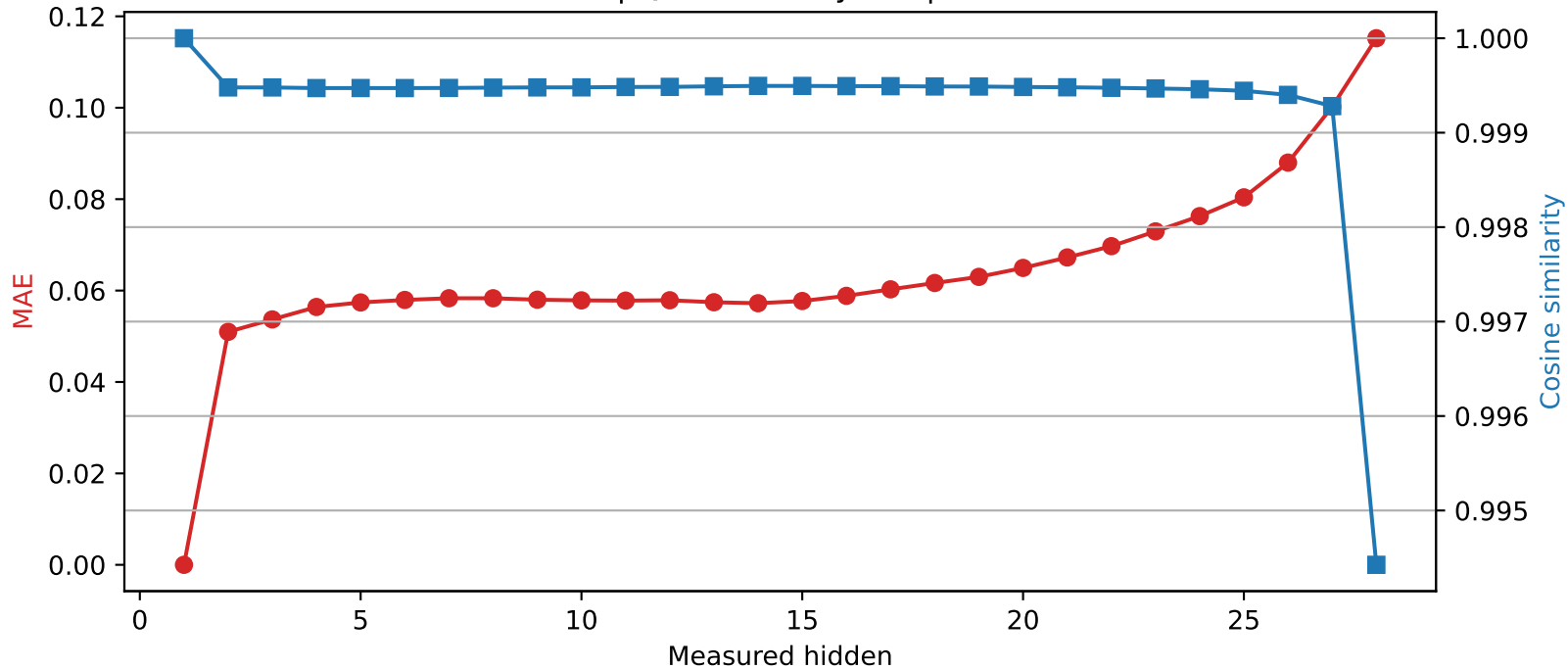
Llama-3.2-3B | Quantized layer 1 | float32 \rightarrow int8
