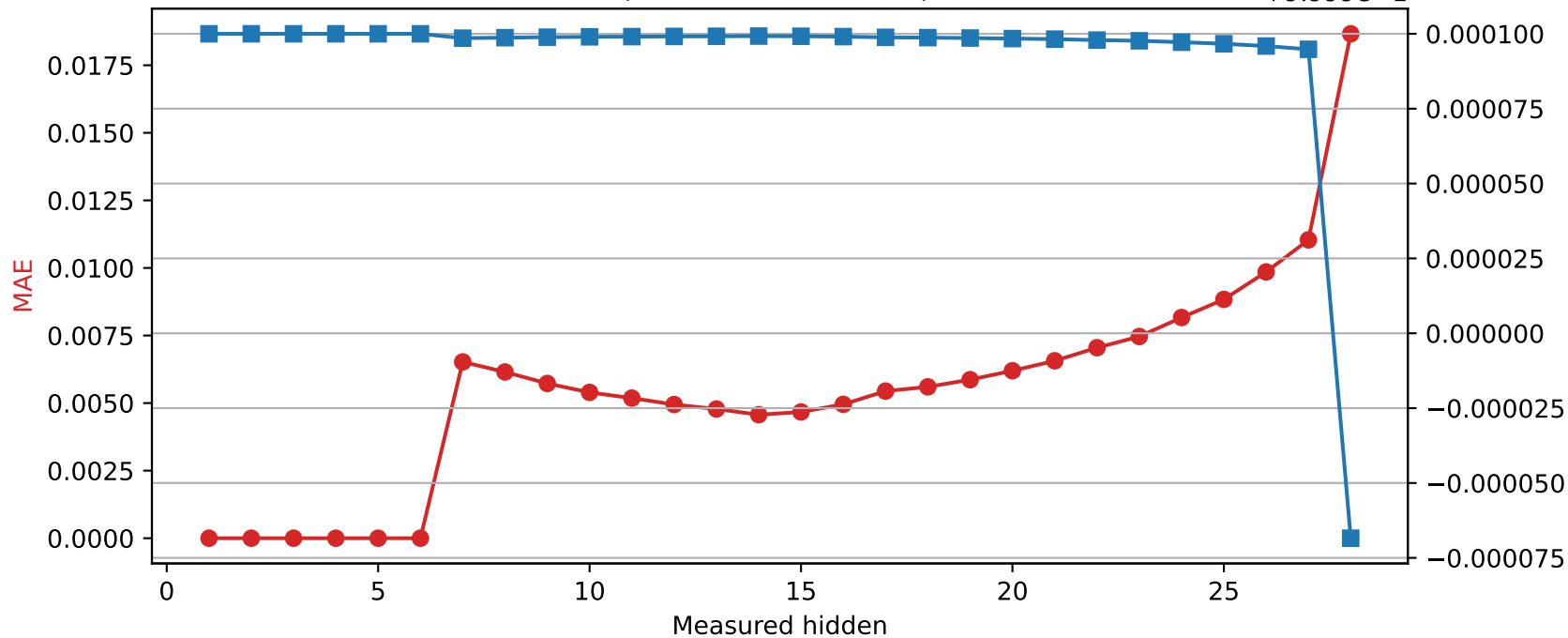
Llama-3.2-3B | Quantized layer 6 | float32 → int8
