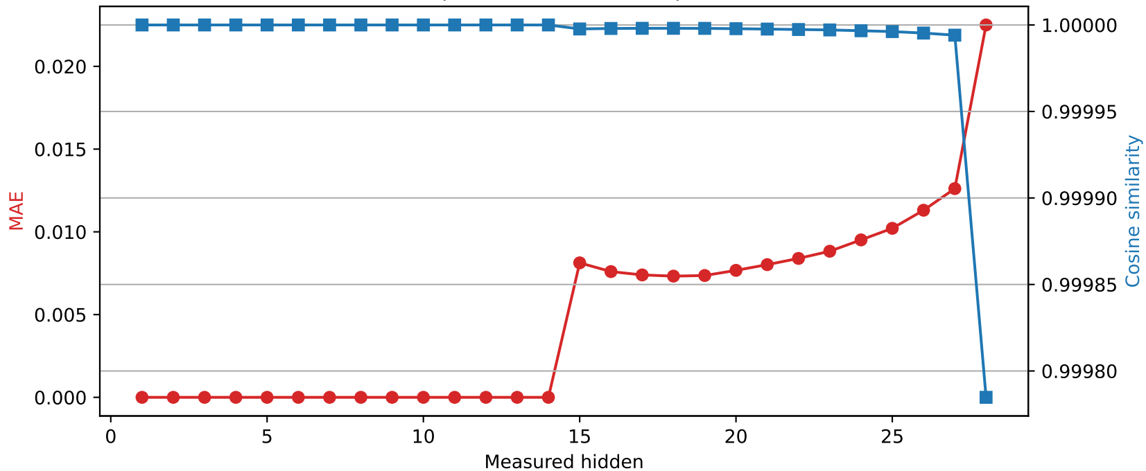
Llama-3.2-3B | Quantized layer 14 | float32 \rightarrow int8
