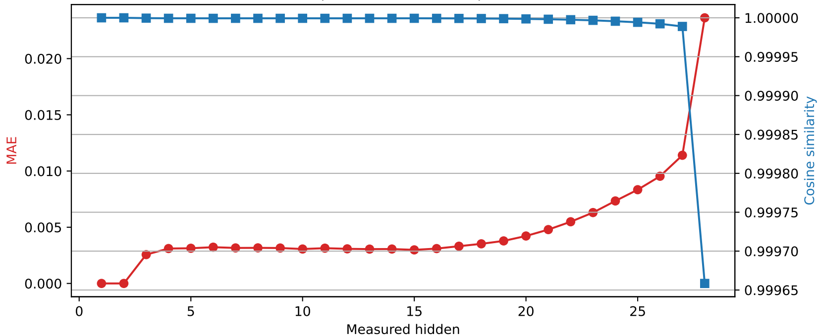
Llama-3.2-3B | Quantized layer 2 | float32 \rightarrow int8
