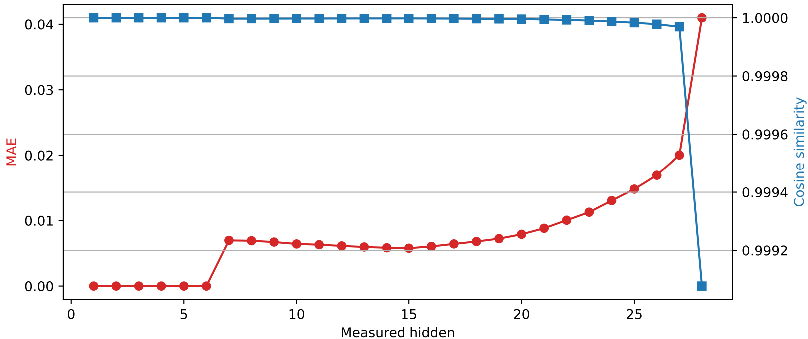
Llama-3.2-3B | Quantized layer 6 | float32 \rightarrow int8
