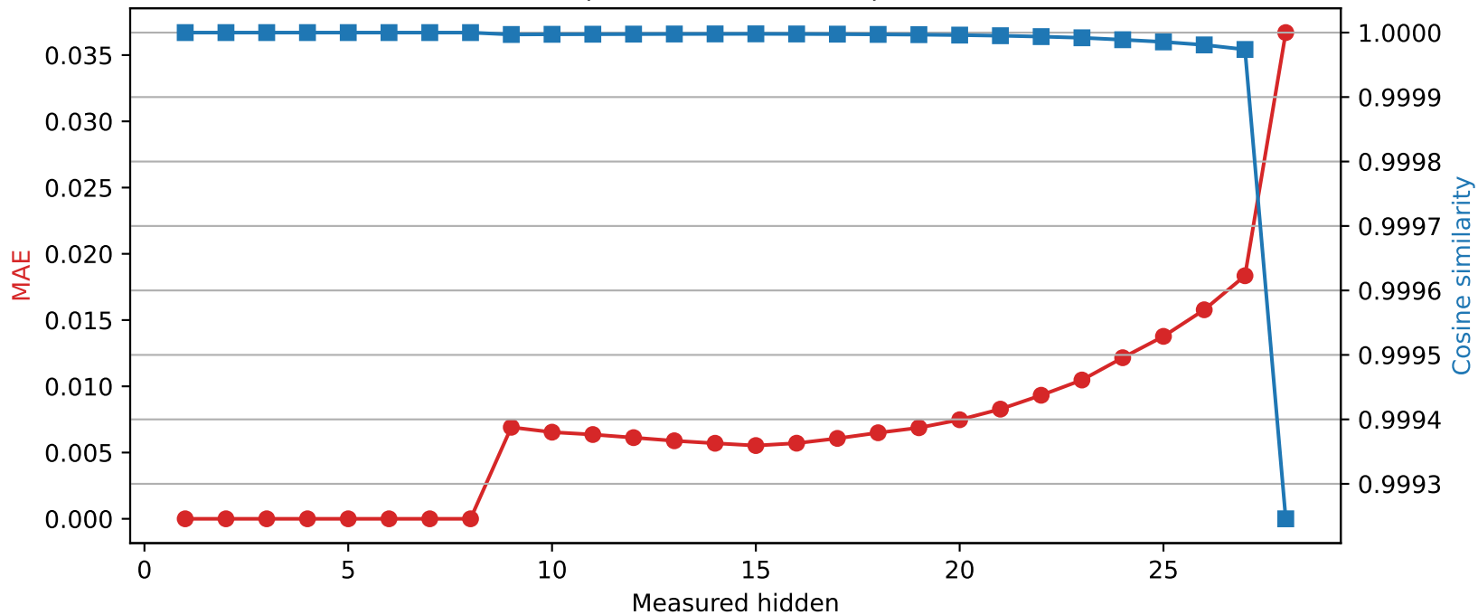
Llama-3.2-3B | Quantized layer 8 | float32 \rightarrow int8
