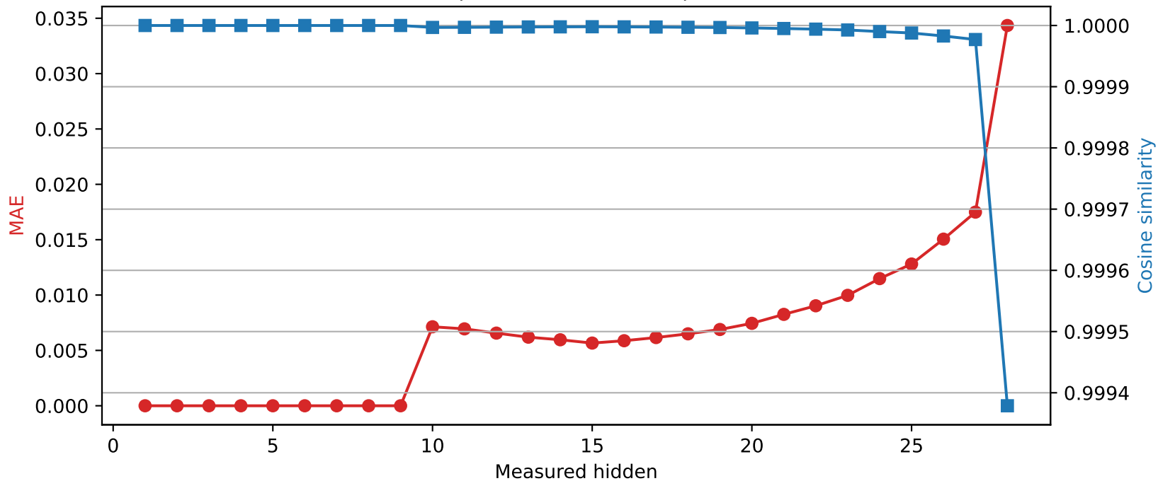
Llama-3.2-3B | Quantized layer 9 | float32 \rightarrow int8
