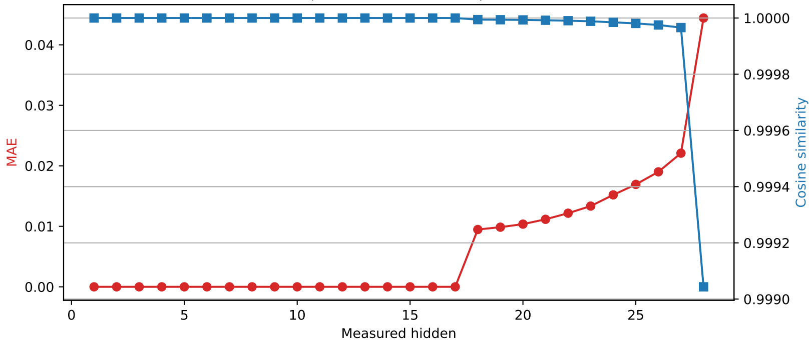
Llama-3.2-3B | Quantized layer 17 | float32 → int8
