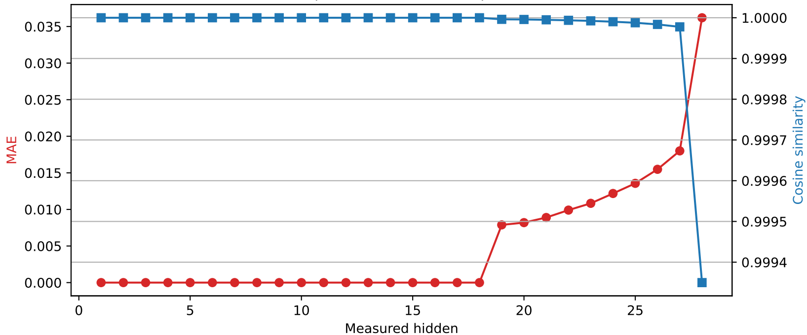
Llama-3.2-3B | Quantized layer 18 | float32 \rightarrow int8
