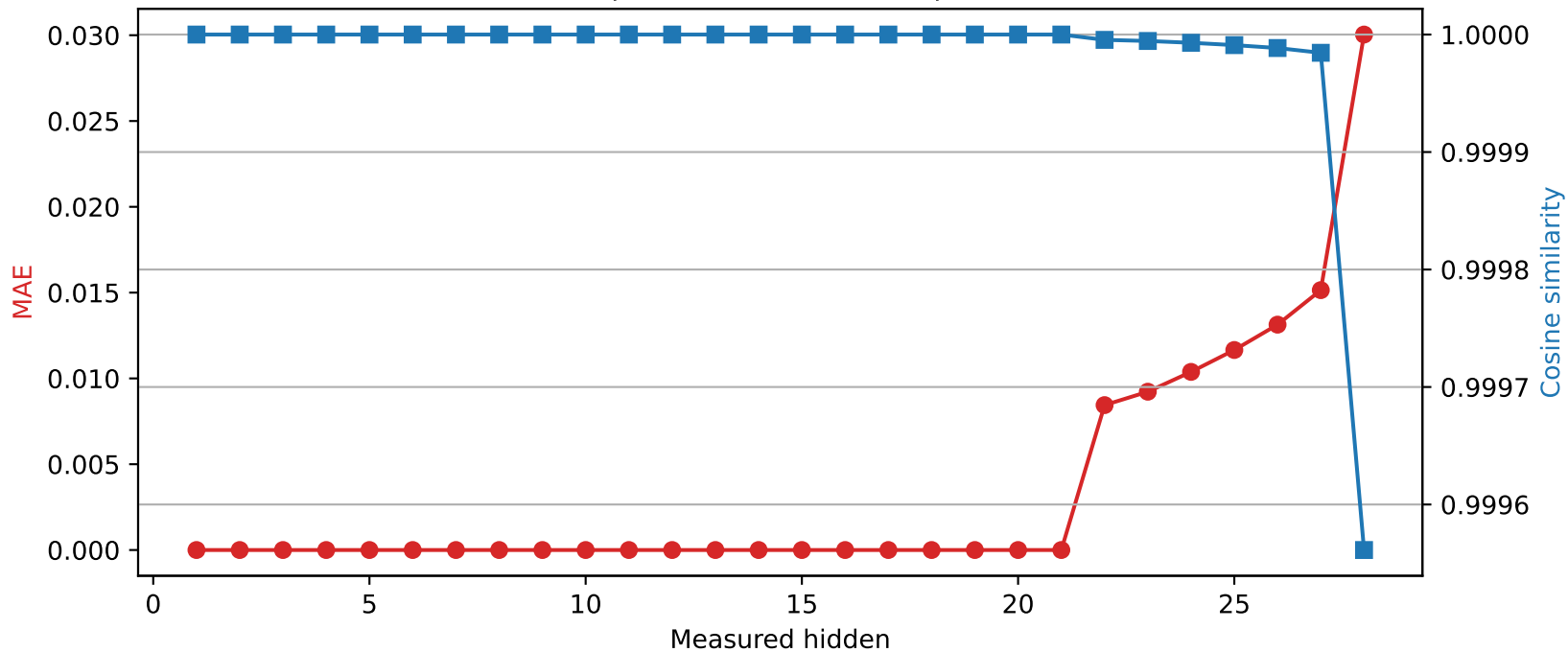
Llama-3.2-3B | Quantized layer 21 | float32 → int8
