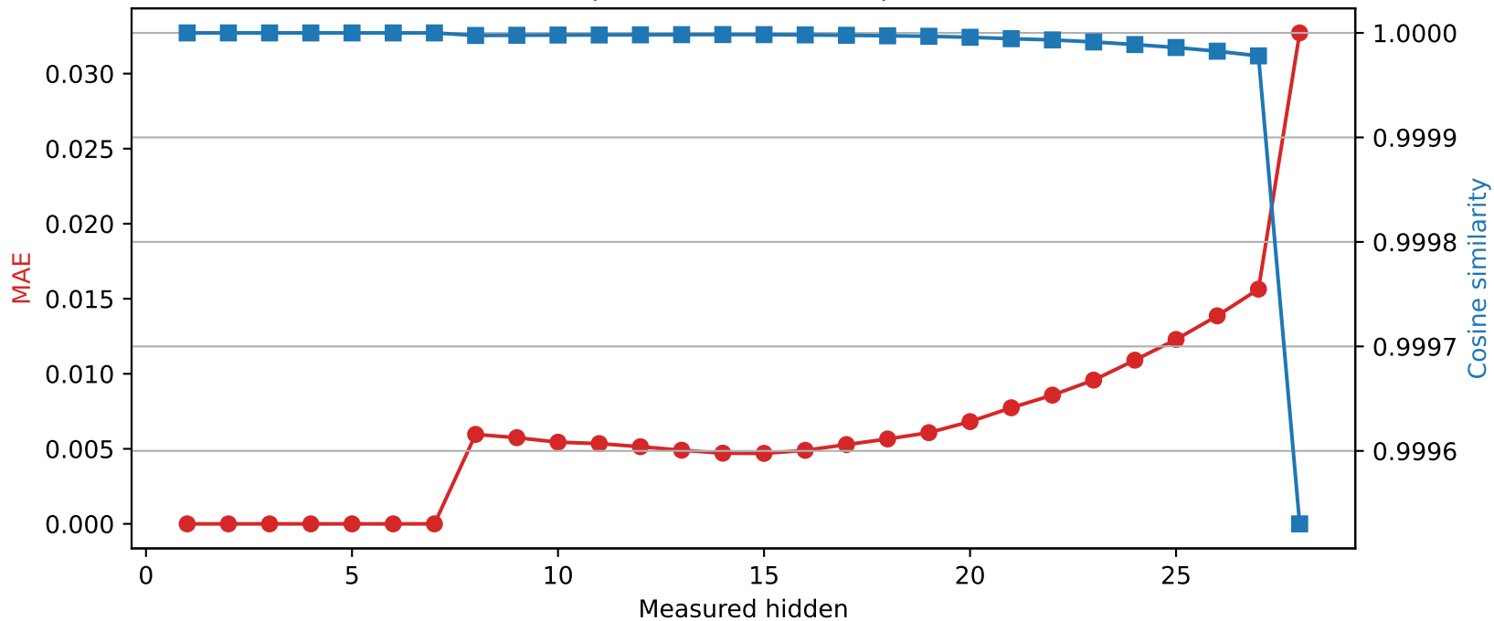
Llama-3.2-3B | Quantized layer 7 | float32 \rightarrow int8
