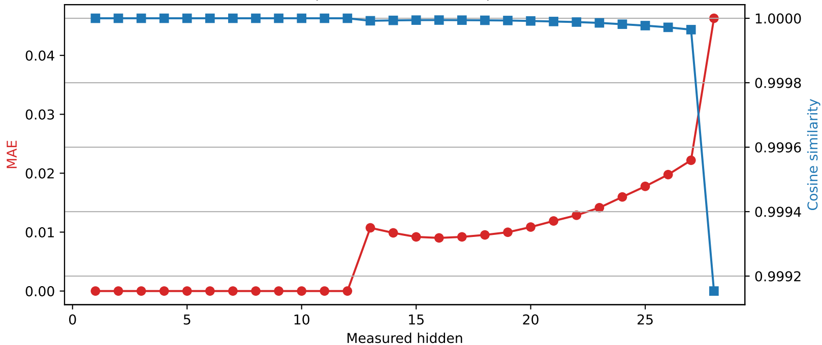
Llama-3.2-3B | Quantized layer 12 | float32 \rightarrow int8
