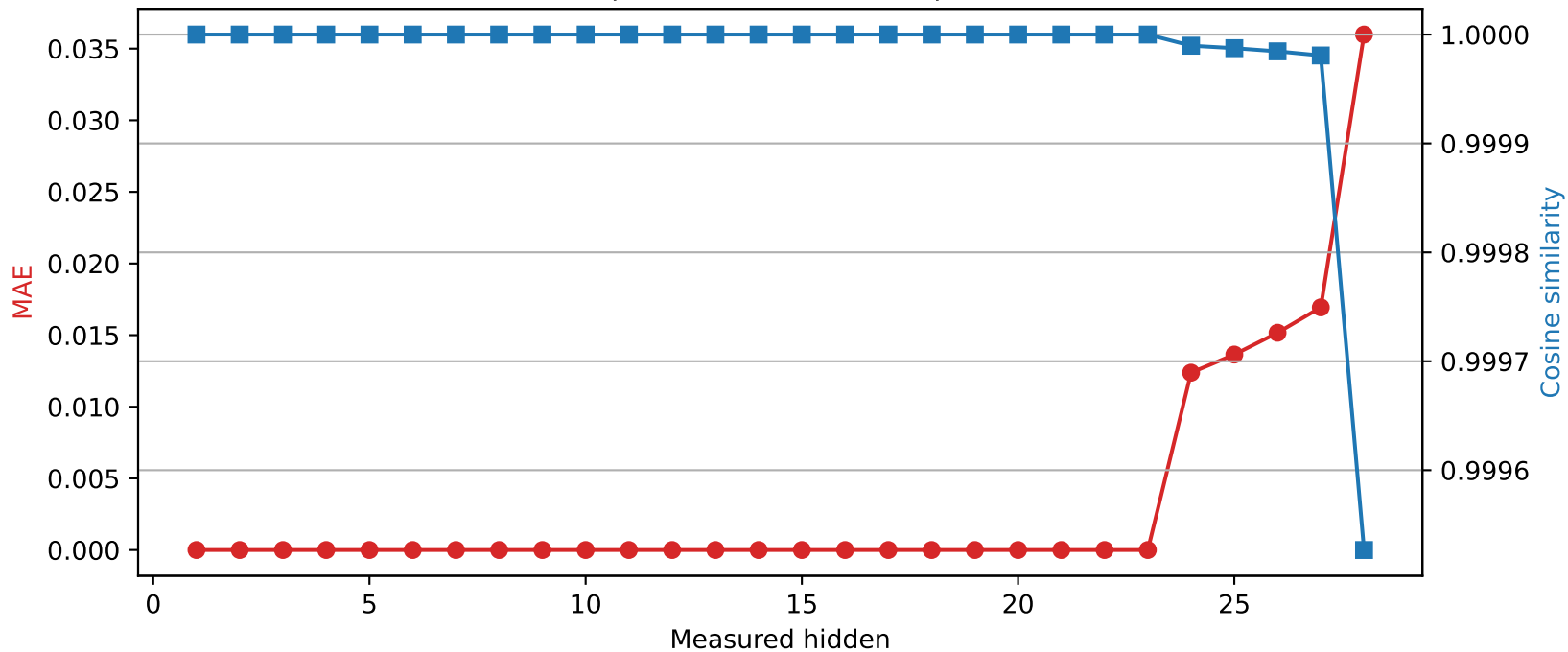
Llama-3.2-3B | Quantized layer 23 | float32 \rightarrow int8
