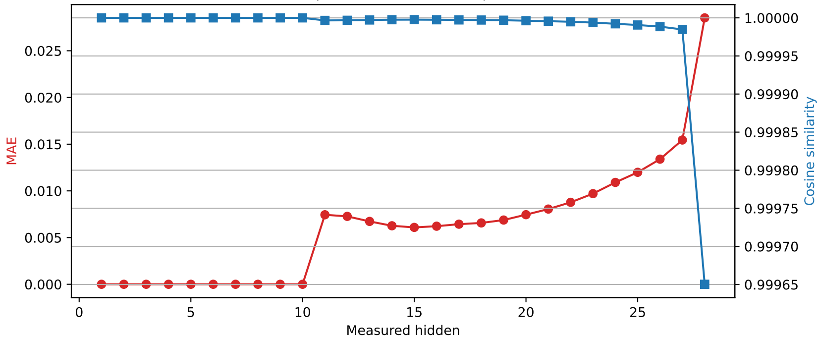
Llama-3.2-3B | Quantized layer 10 | float32 → int8
