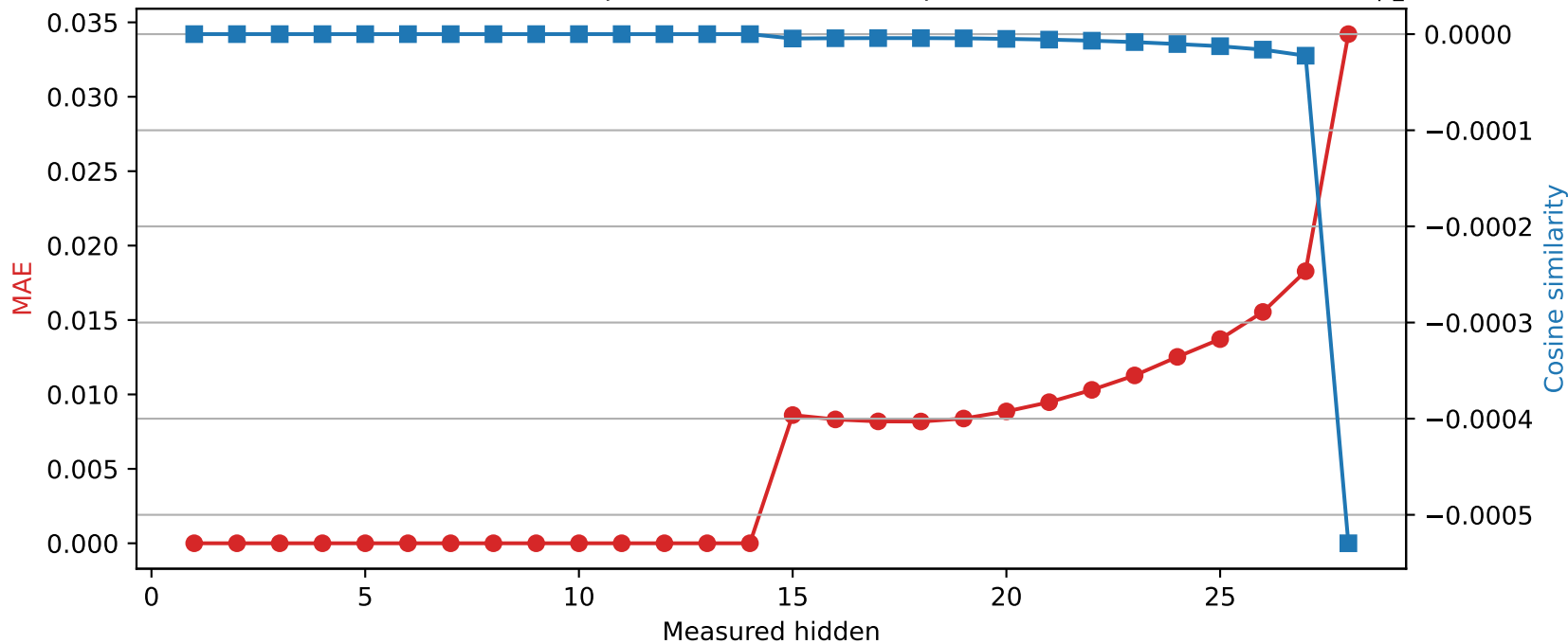
Llama-3.2-3B | Quantized layer 14 | float32 → int8
