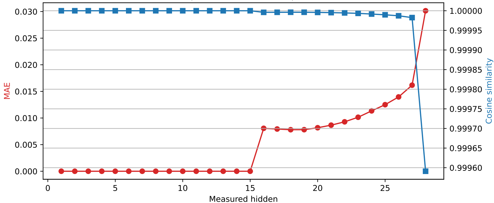
Llama-3.2-3B | Quantized layer 15 | float32 → int8
