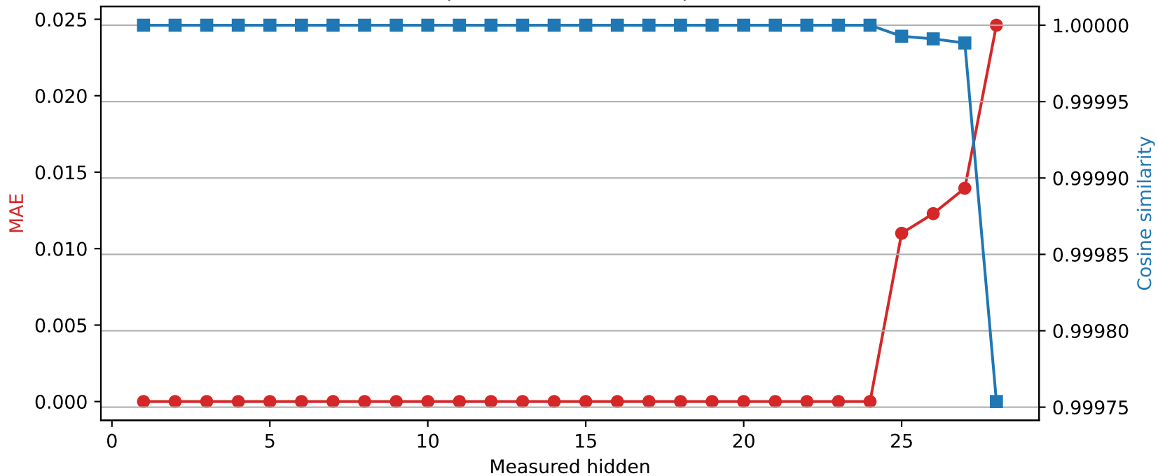
Llama-3.2-3B | Quantized layer 24 | float32 → int8
