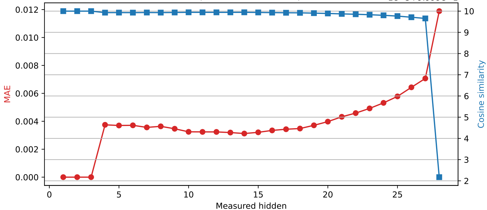
Llama-3.2-3B | Quantized layer 3 | float32 → int8
