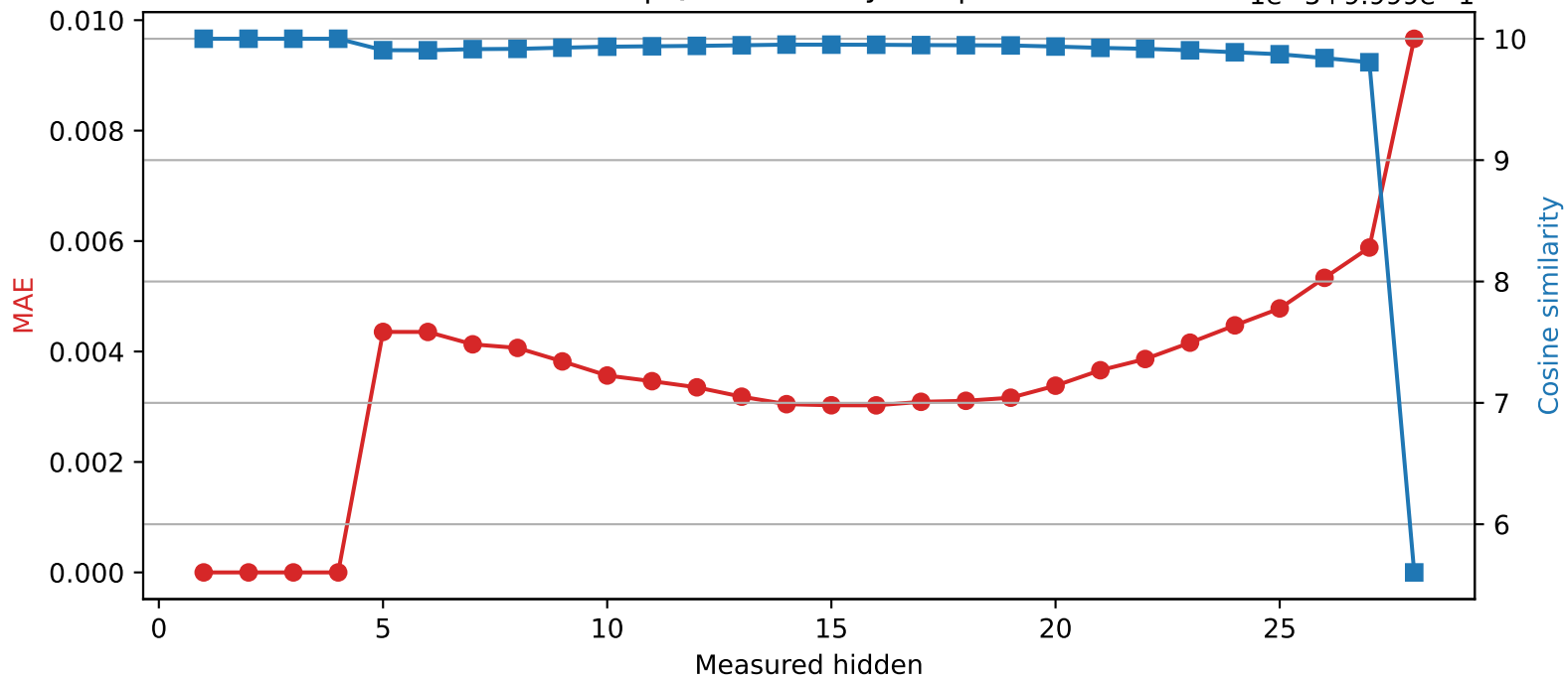
Llama-3.2-3B | Quantized layer 4 | float32 → int8
