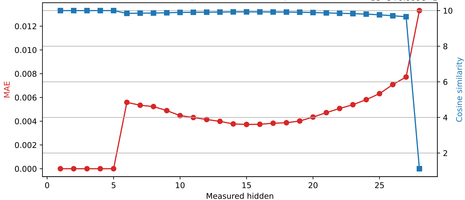
Llama-3.2-3B | Quantized layer 5 | float32 → int8
