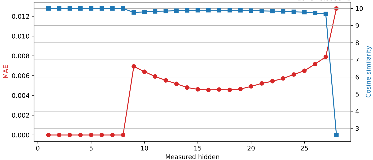
Llama-3.2-3B | Quantized layer 8 | float32 → int8
