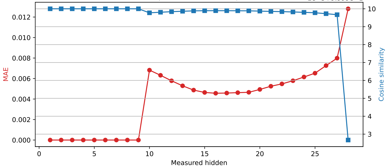
Llama-3.2-3B | Quantized layer 9 | float32 → int8
