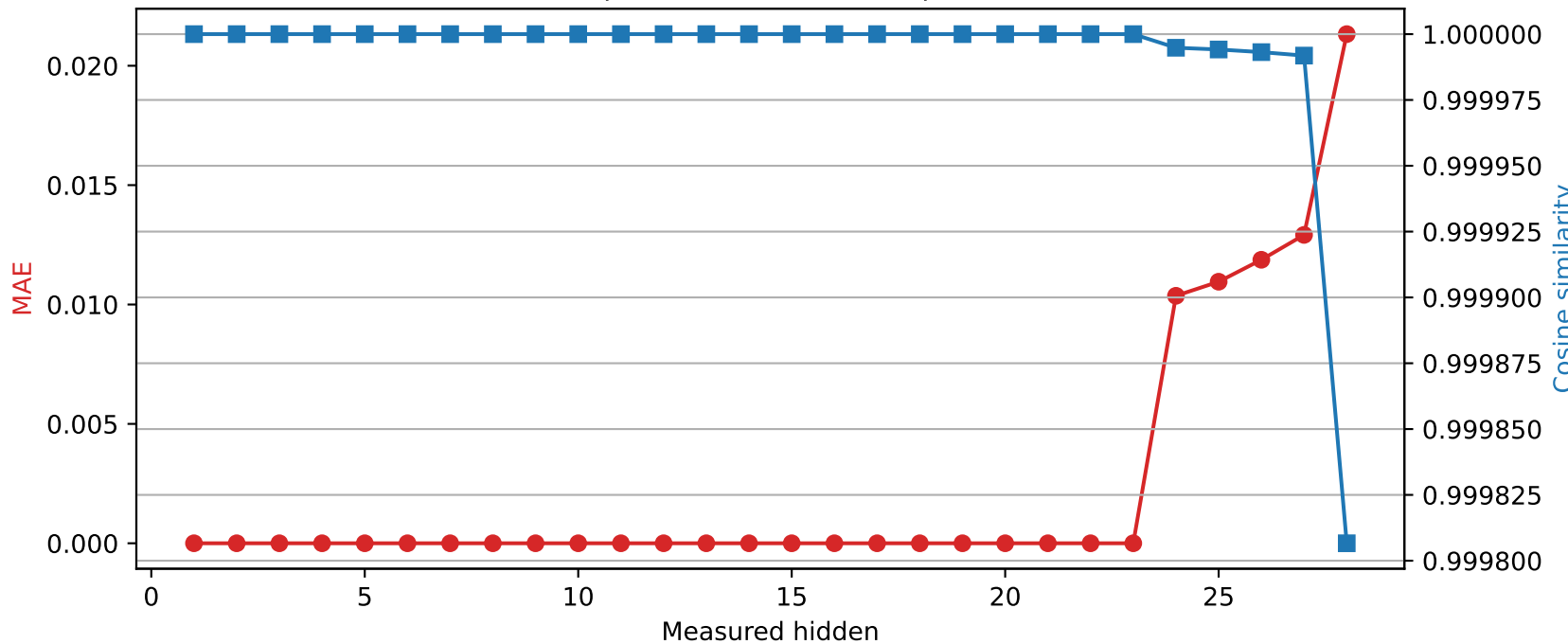
Llama-3.2-3B | Quantized layer 23 | float32 \rightarrow int8
