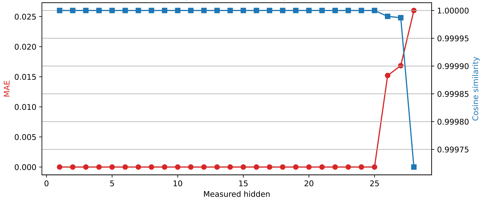
Llama-3.2-3B | Quantized layer 25 | float32 \rightarrow int8
