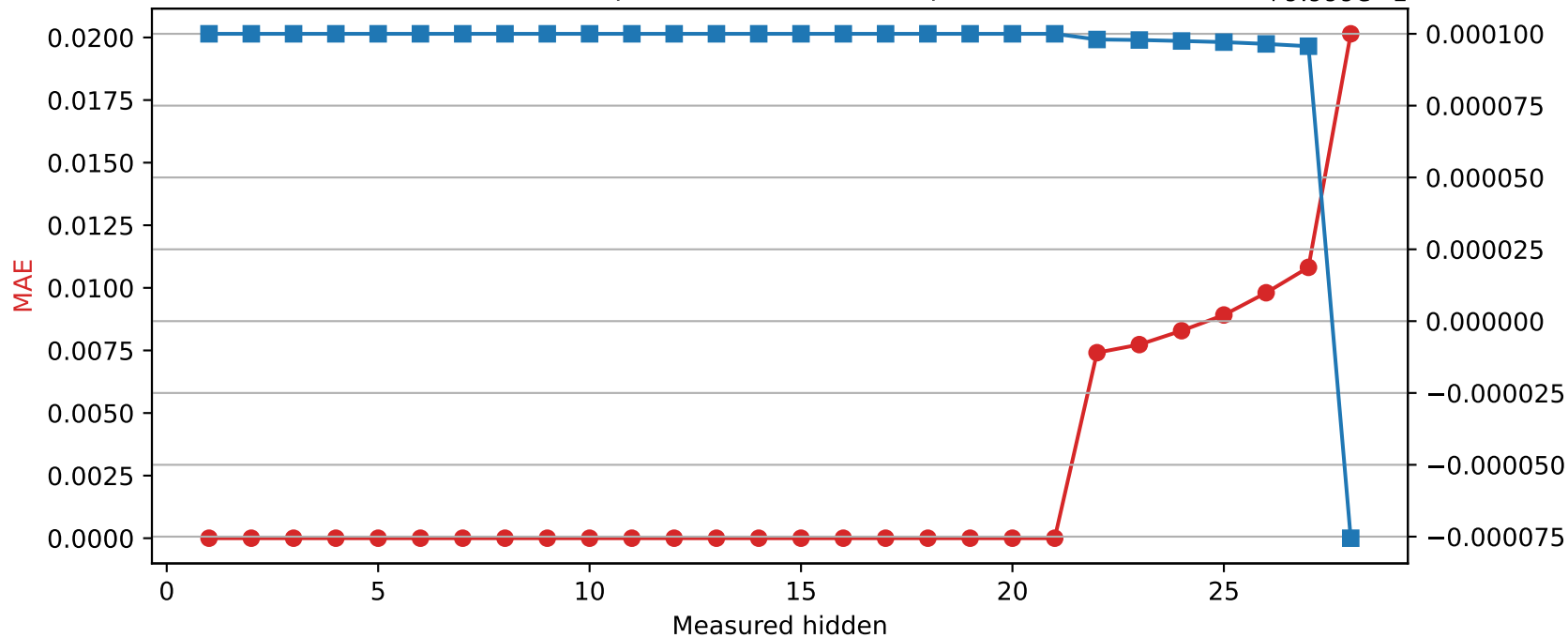
Llama-3.2-3B | Quantized layer 21 | float64 → int8
