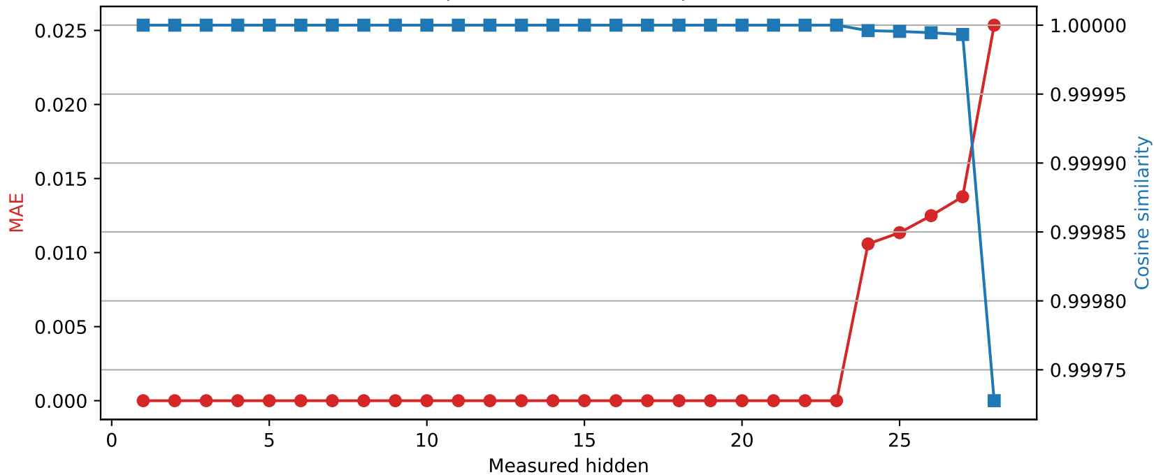
Llama-3.2-3B | Quantized layer 23 | float64 → int8
