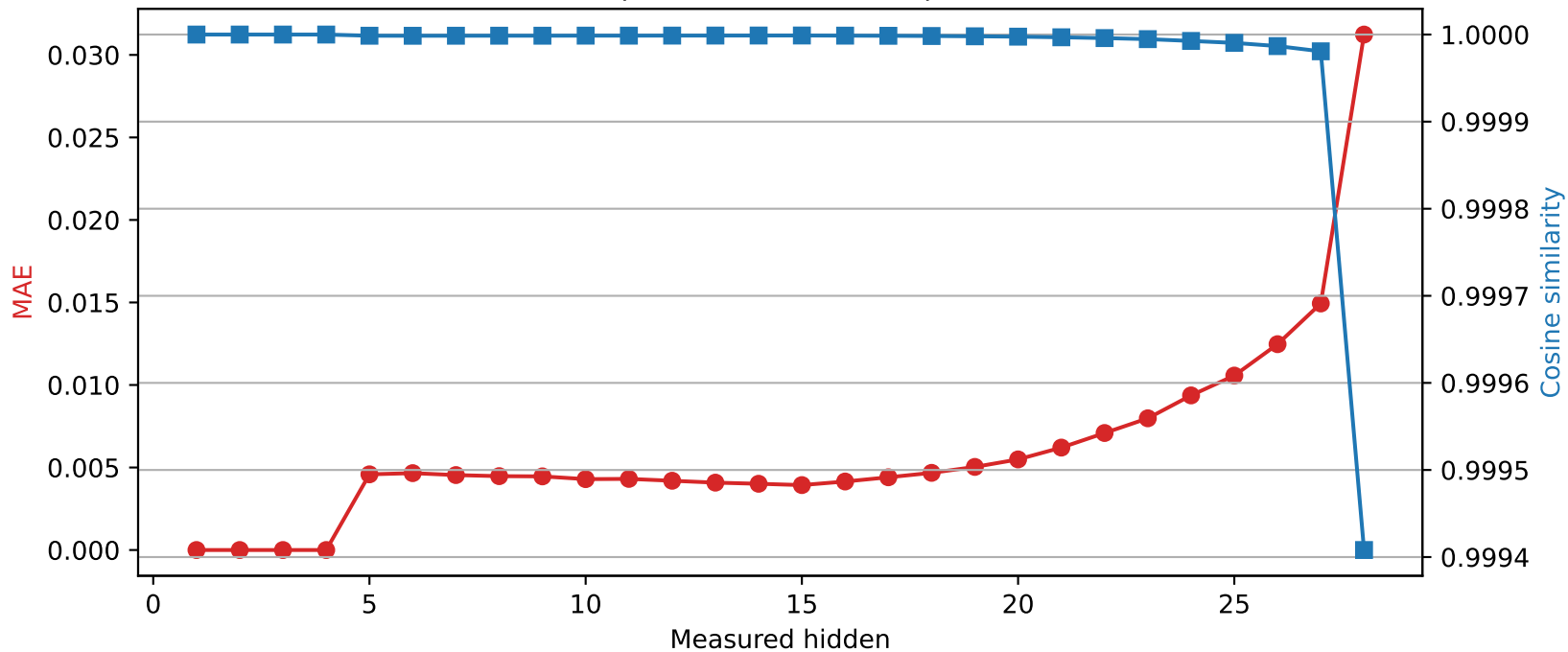
Llama-3.2-3B | Quantized layer 4 | float64 → int8
