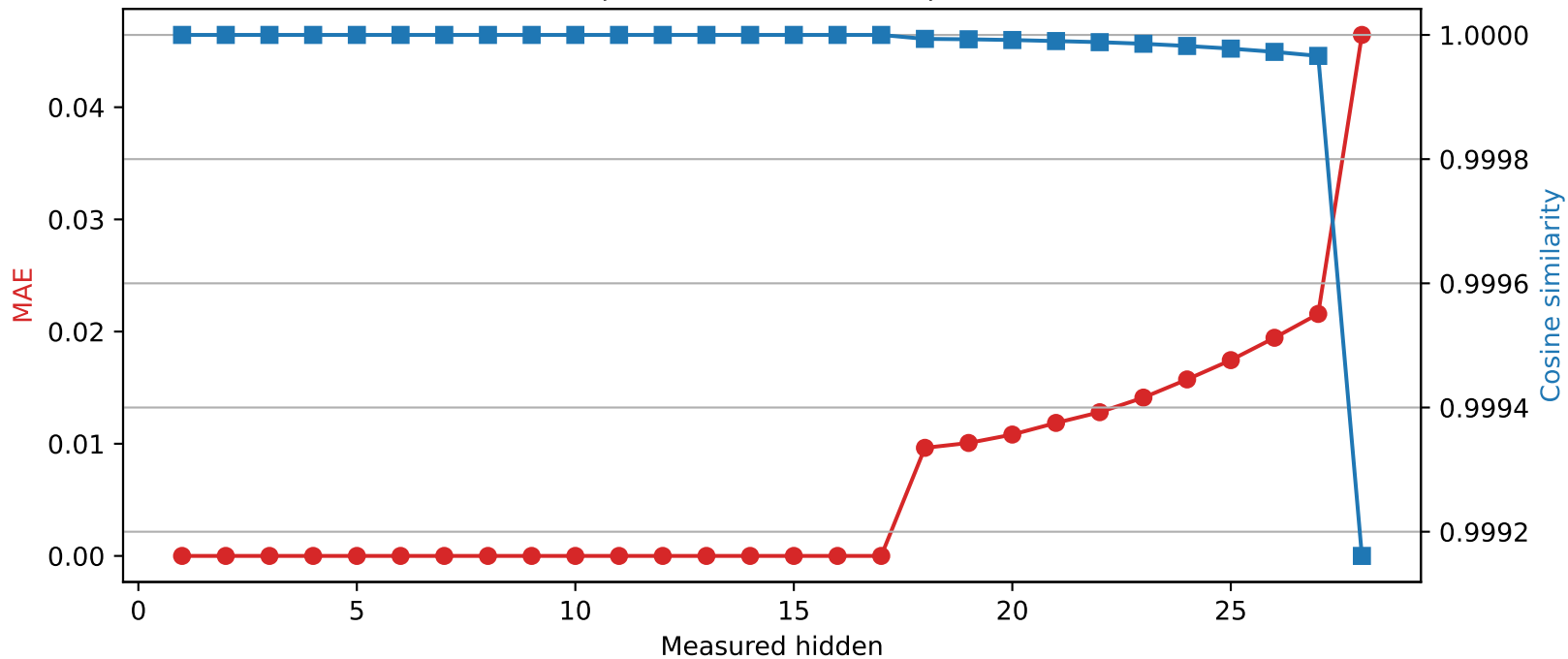
Llama-3.2-3B | Quantized layer 17 | float64 \rightarrow int8
