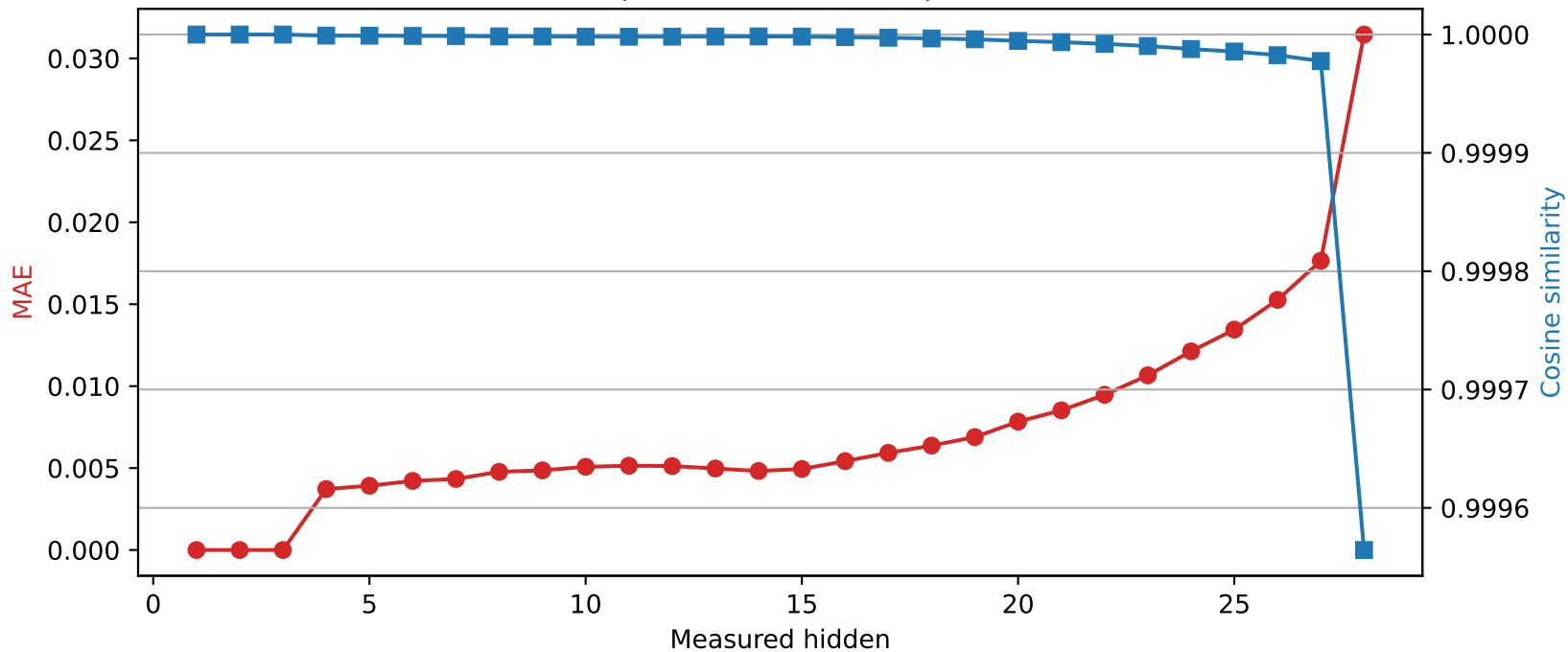
Llama-3.2-3B | Quantized layer 3 | float64 → int8
