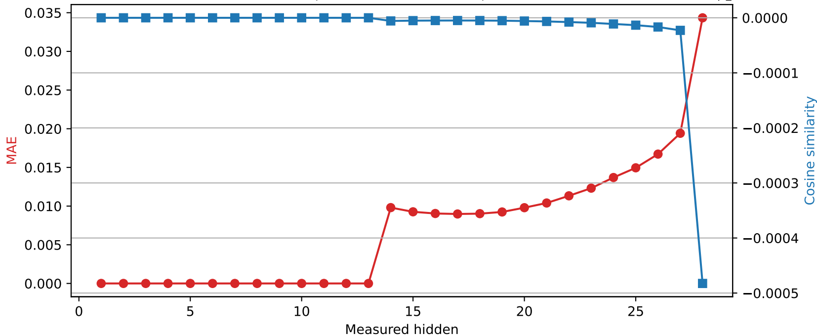
Llama-3.2-3B | Quantized layer 13 | float64 → int8
