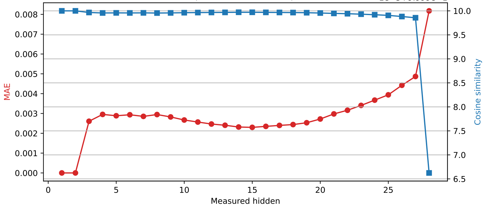
Llama-3.2-3B | Quantized layer 2 | float64 → int8
