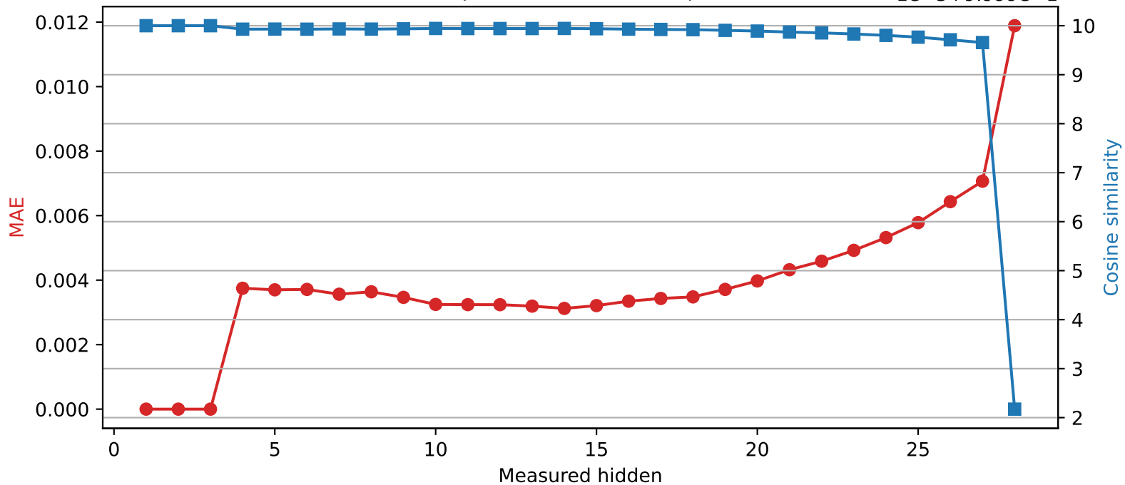
Llama-3.2-3B | Quantized layer 3 | float64 → int8
