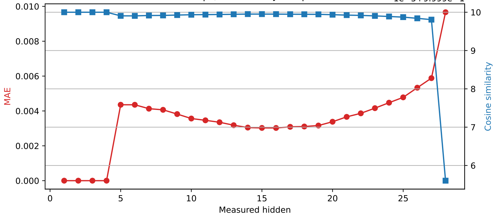
Llama-3.2-3B | Quantized layer 4 | float64 → int8
