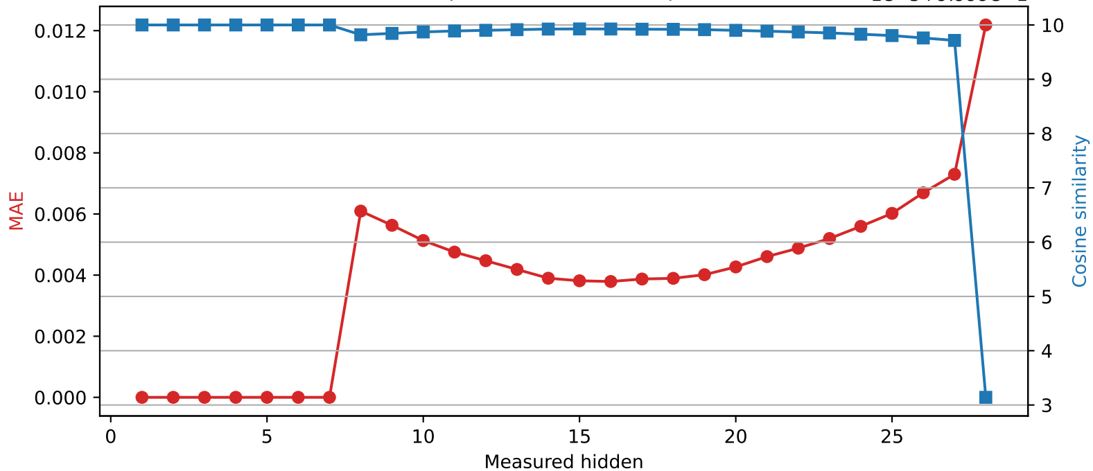
Llama-3.2-3B | Quantized layer 7 | float64 → int8
