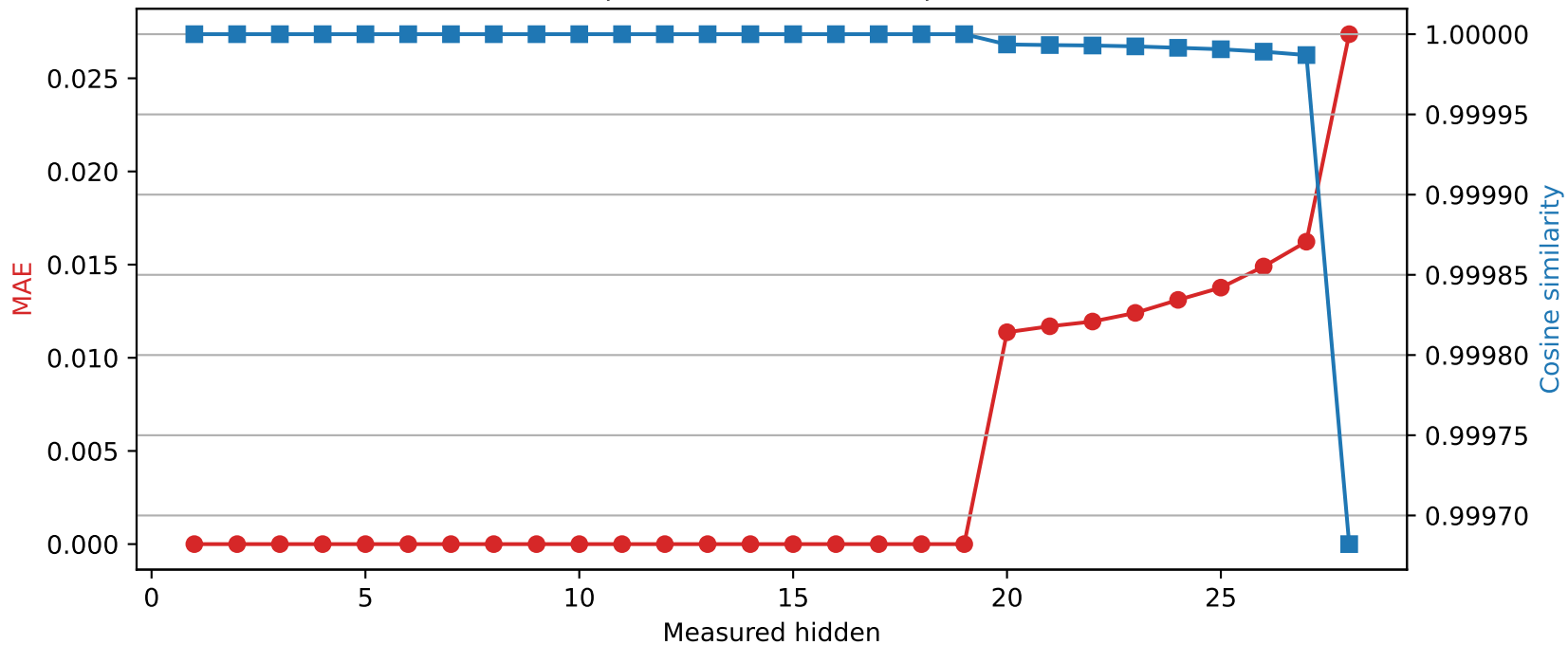
Llama-3.2-3B | Quantized layer 19 | float64 → int8
