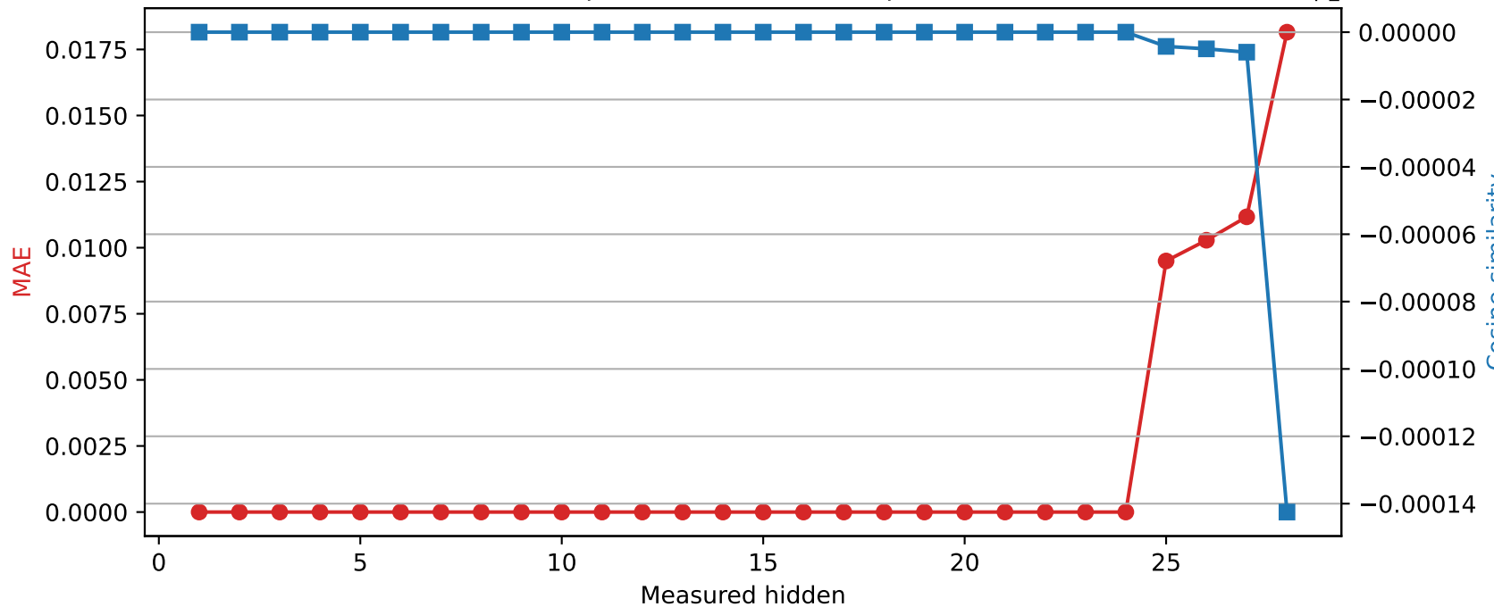
Llama-3.2-3B | Quantized layer 24 | float64 → int8
