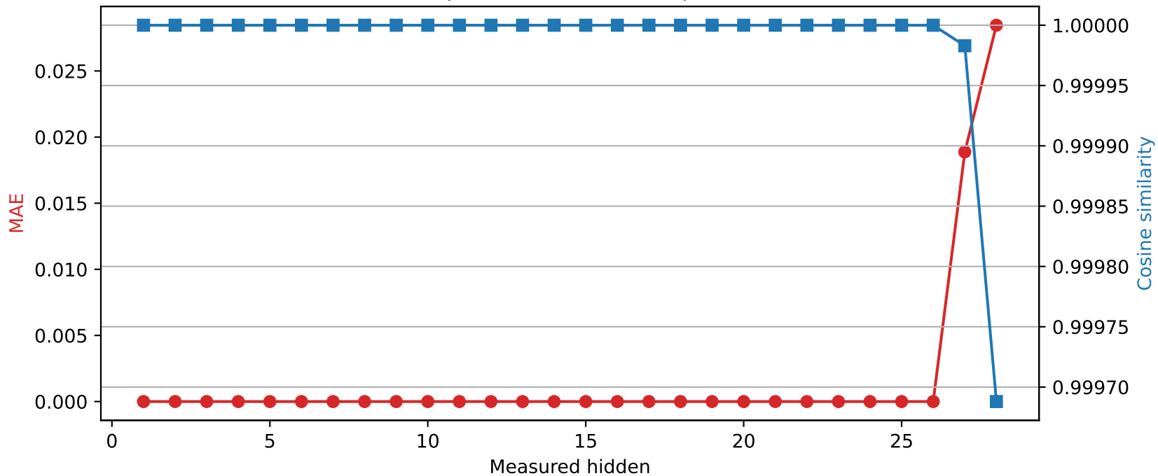
Llama-3.2-3B | Quantized layer 26 | float64 → int8
