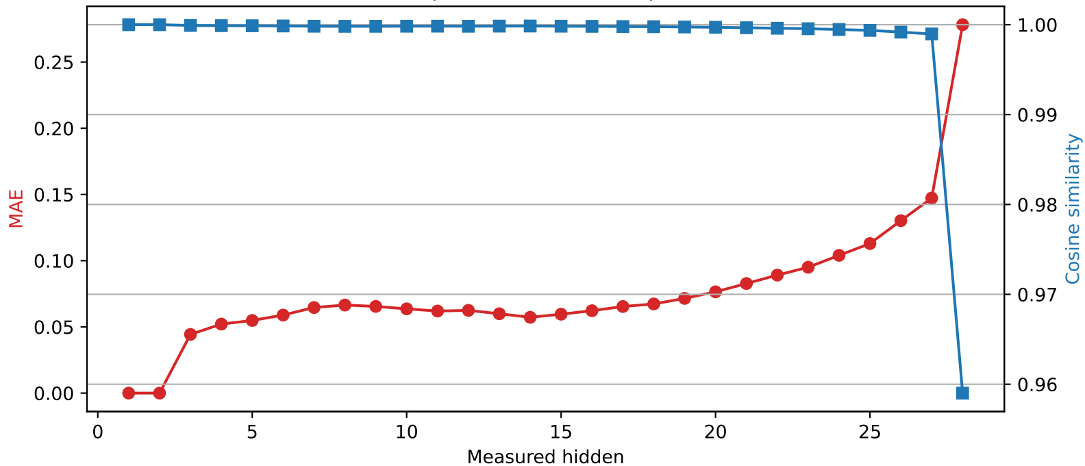
Llama-3.2-3B | Quantized layer 2 | float16 → int4
