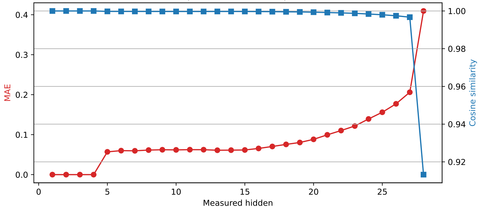
Llama-3.2-3B | Quantized layer 4 | float16 \rightarrow int4
