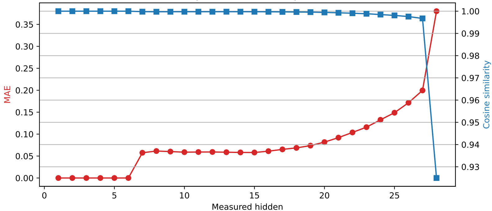
Llama-3.2-3B | Quantized layer 6 | float16 \rightarrow int4
