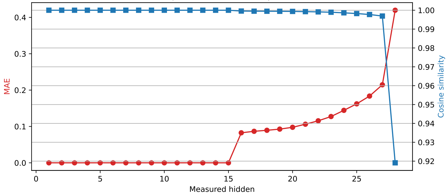
Llama-3.2-3B | Quantized layer 15 | float16 \rightarrow int4
