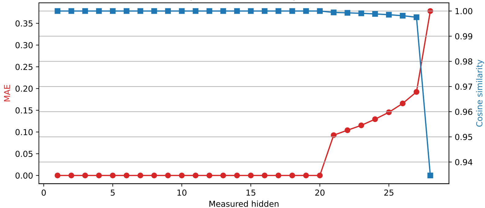
Llama-3.2-3B | Quantized layer 20 | float16 → int4
