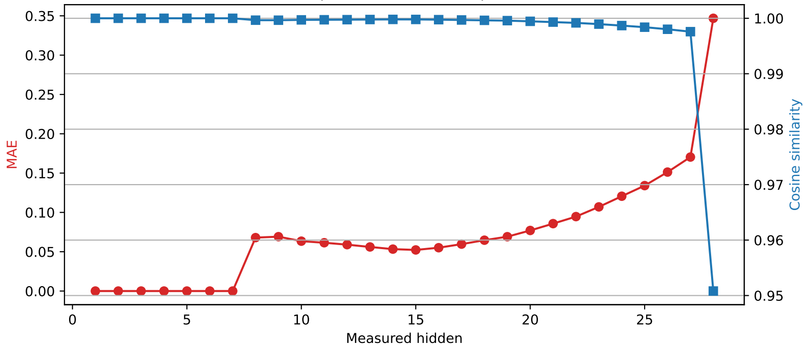
Llama-3.2-3B | Quantized layer 7 | float16 \rightarrow int4
