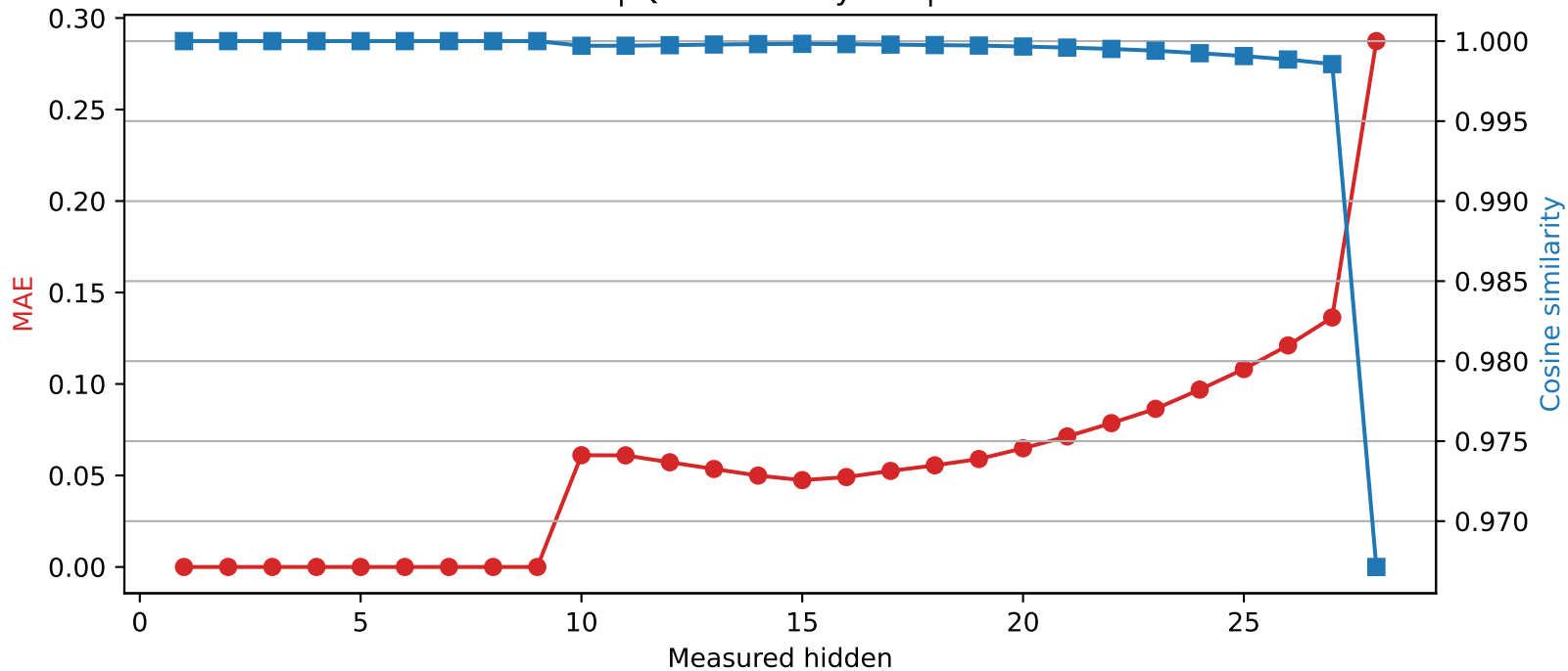
Llama-3.2-3B | Quantized layer 9 | float16 \rightarrow int4
