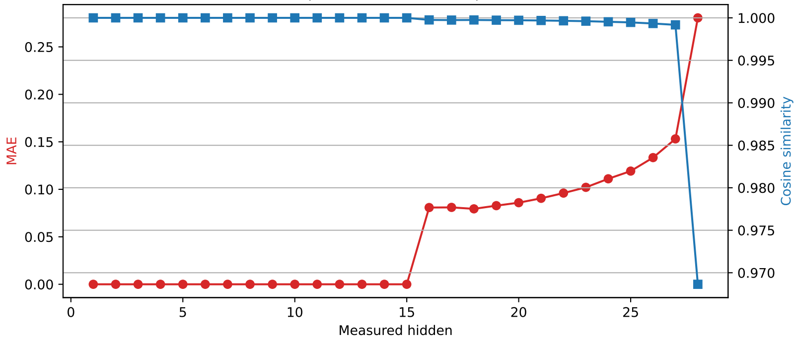
Llama-3.2-3B | Quantized layer 15 | float32 \rightarrow int4
