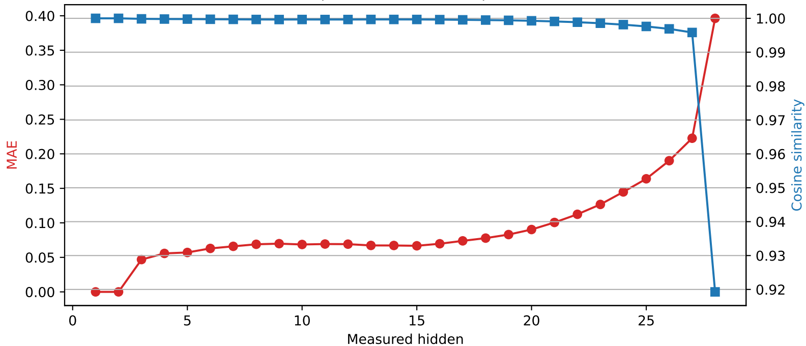
Llama-3.2-3B | Quantized layer 2 | float32 → int4
