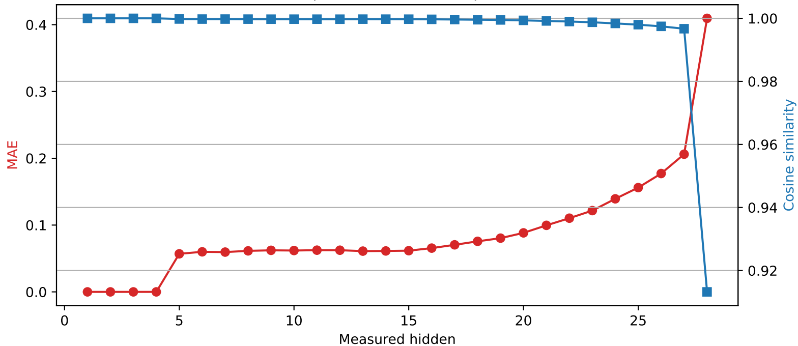
Llama-3.2-3B | Quantized layer 4 | float32 → int4
