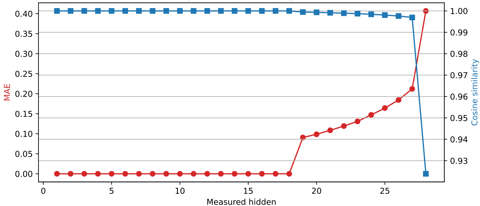
Llama-3.2-3B | Quantized layer 18 | float32 → int4
